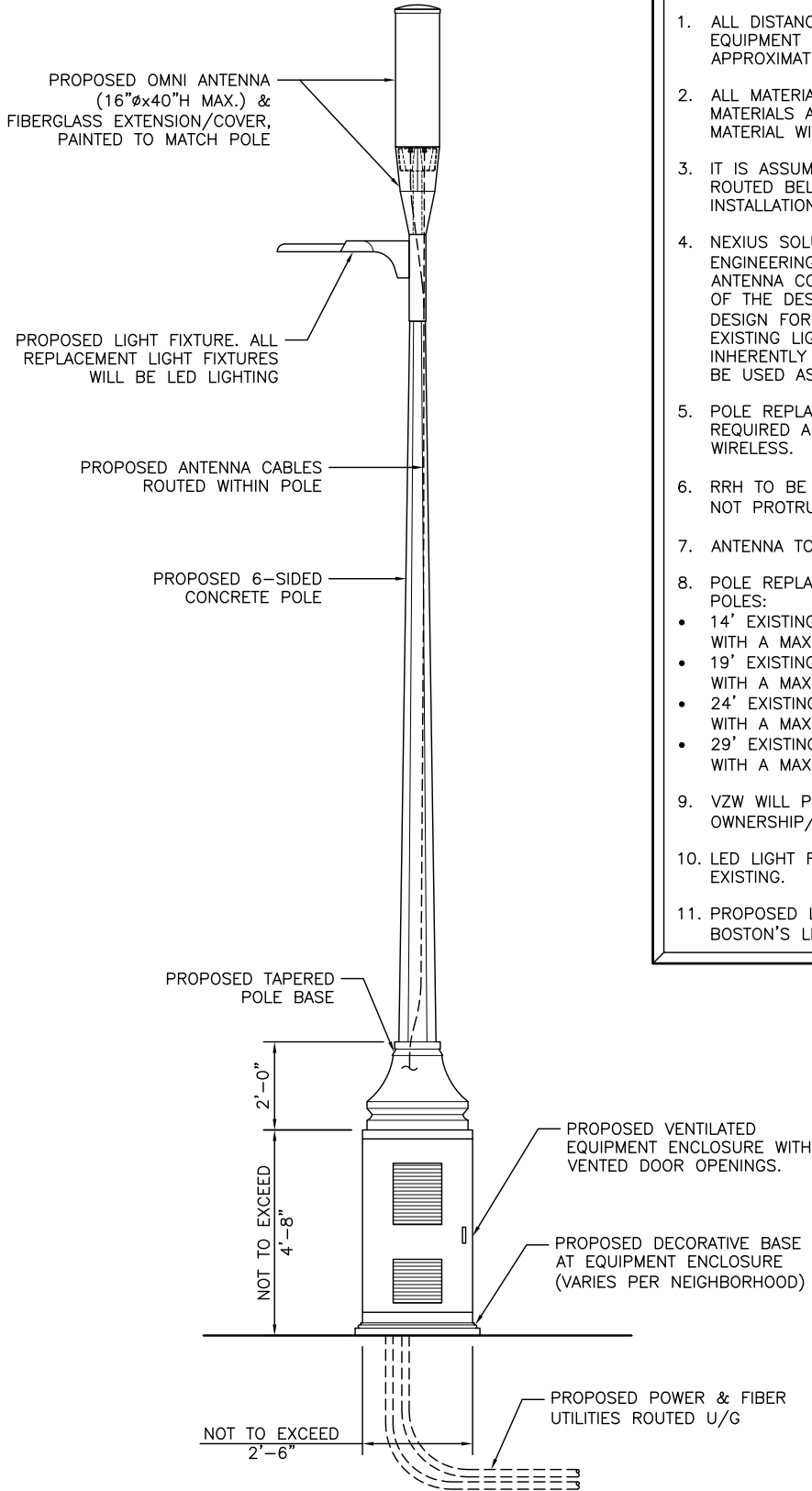
AERIATA CONCRETE LIGHT POLE W/ RRH CONCEALMENT
