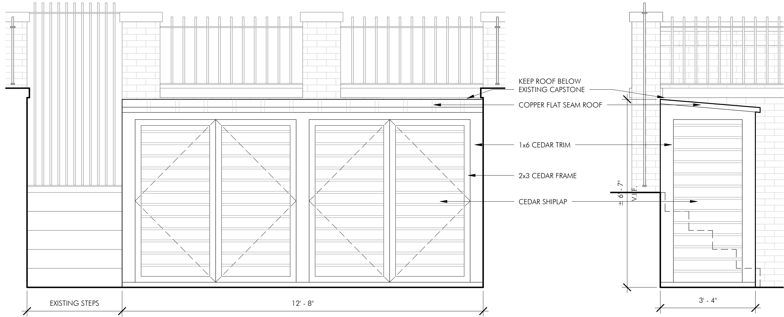
SHED - FRONT ELEVATION
