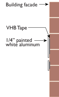
MK MOUNTING DETAIL SCALE: 1-1/2" = 1'-0"
