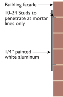
COR MOUNTING DETAIL SCALE: 1-1/2" = 1'-0"
