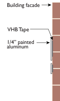
MK MOUNTING DETAIL SCALE: 1-1/2" = 1'-0"
