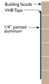
COR MOUNTING DETAIL SCALE: 1-1/2" = 1'-0"
