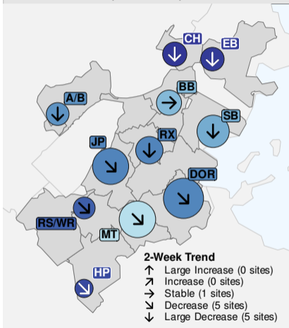
COVID-19 Wastewater Levels & Trends (03-Mar-2024)
