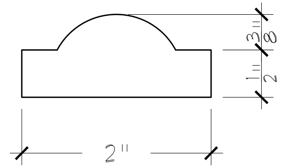
3 PROPOSED RAILING PROFILE FULL: 12" = 1'-0", HALF: 6" = 1'-0"
