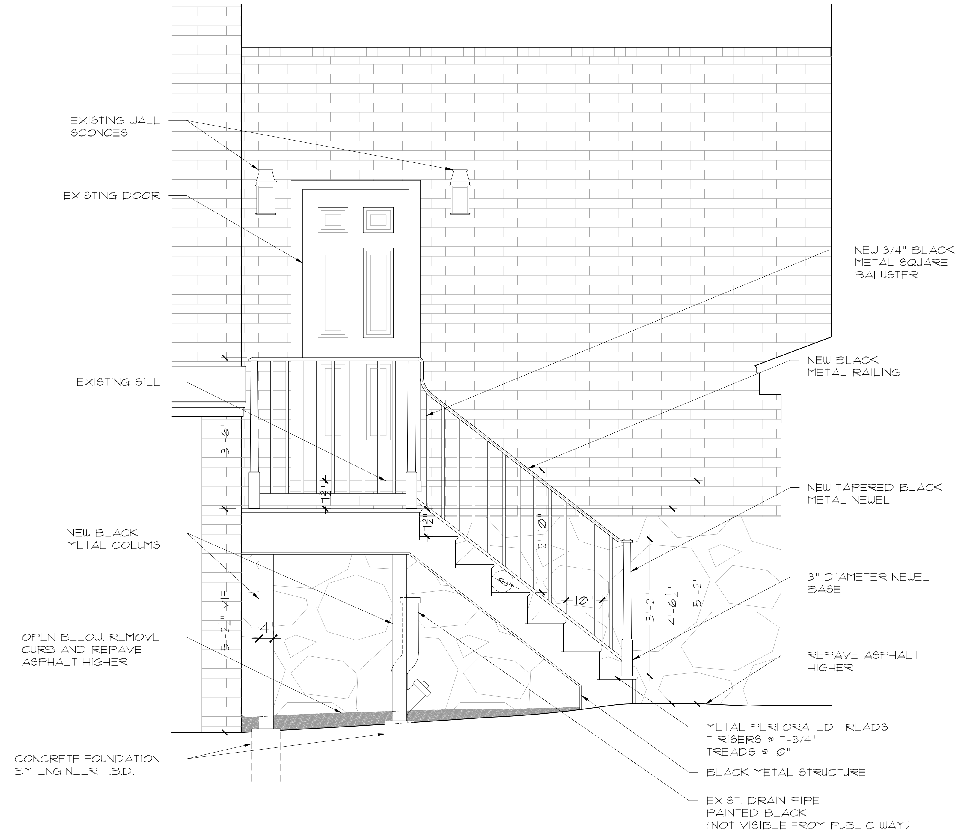
PROPOSED EXTERIOR METAL STAIR
